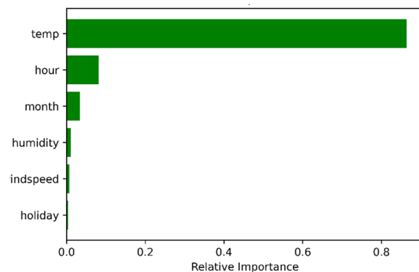
Figure 5. Feature importance using the mean decrease in impurity.
